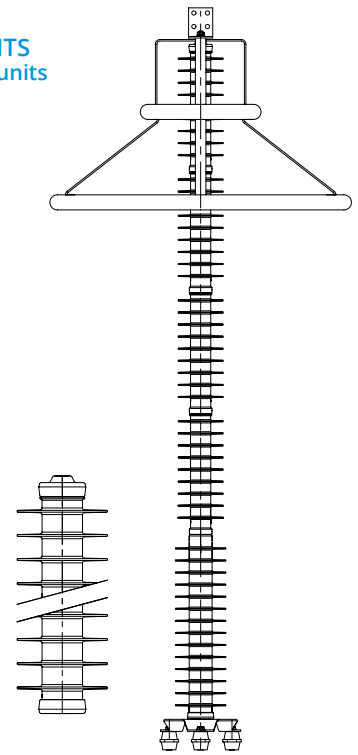
TC with grating ring
