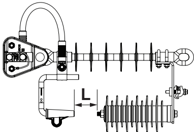
SDI46.824 + (SDP5.2+SO181.6)
