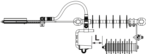
SDI46.824 + (SDP5.2+SO255/SO256)
