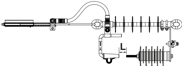
SDI46.824 + (SDP5.2+SO255/SO256)
