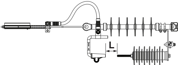
SDI46.824 + (SDP5.2+SO181.6)
